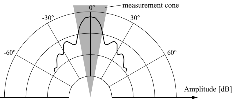
Figure 4.7 Typical intensity distribution of an ultrasonic sensor.
