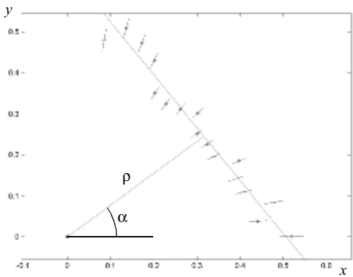
Figure 4.37 Extracted line from laser range measurements (+). The small lines at each measurement point represent the measurement uncertainty \sigma that is proportional to the square of the measurement distance.
