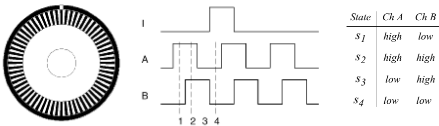
Figure 4.2 Quadrature optical wheel encoder: The observed phase relationship between channel A and B pulse trains are used to determine the direction of the rotation. A single slot in the outer track generates a reference (index) pulse per revolution.
