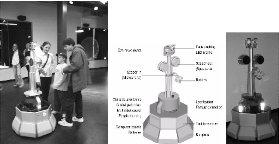
Figure 1.7 Tour-guide robots are able to interact and present exhibitions in an educational way [48, 118, 132, 143,]. Ten Roboxes have operated during 5 months at the Swiss exhibition EXPO.02, meeting hundreds of thousands of visitors. They were developed by EPFL [132] ( http://robotics.epfl.ch ) and commercialized by BlueBotics ( http://www.bluebotics.ch ).
