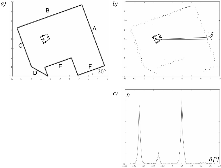
Figure 4.39 Angle histogram [155].
