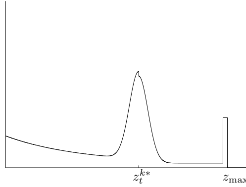
Figure 6.3 “Pseudo-density” of a typical mixture distribution p(z_t^k | x_t, m) .
