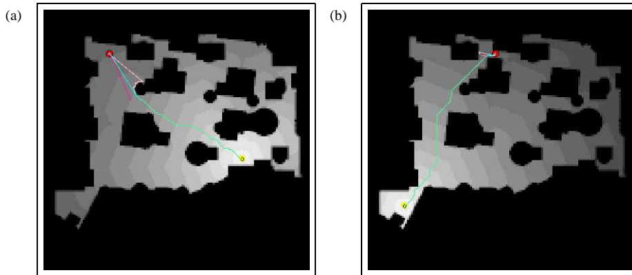
Figure 15.2 Example of value iteration over state spaces in robot motion. Obstacles are shown in black. The value function is indicated by the grayly shaded area. Greedy action selection with respect to the value function lead to optimal control, assuming that the robot's pose is observable. Also shown in the diagrams are example paths obtained by following the greedy policy.
